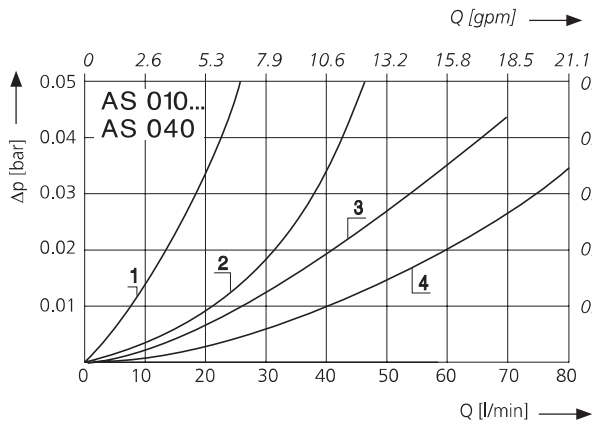
D1 Pressure drop as a function of the flow volume at \nu = 35 \text{ mm}^2/\text{s} / 162 \text{ SUS}
