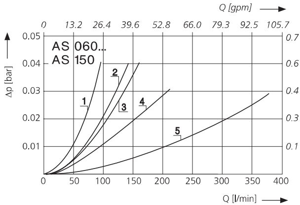
D2 Pressure drop as a function of the flow volume at \nu = 35 \text{ mm}^2/\text{s} / 162 \text{ SUS}
